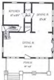
First Floor Plan—Shadow Lawn
