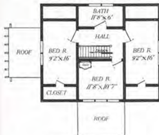
Second Floor Plan—The Strathmore
