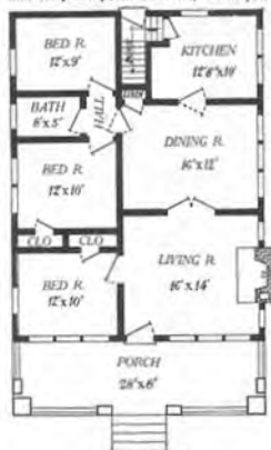
Floor Plan—The Franklin
