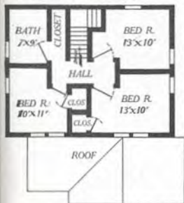
Second Floor Plan—The Georgia No. 2
