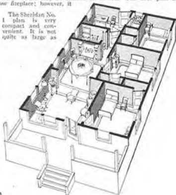
Floor Plan—The Sheridan No. 1
