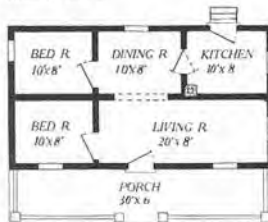
Floor Plan The Gretna No. 2.
