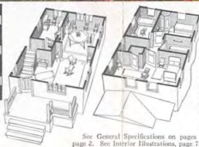
Second Floor Plan The Venus No. 2
