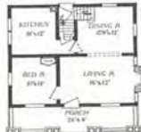
First Floor Plan—The Detroit
