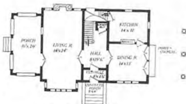
First Floor Plan—The Brentwood
