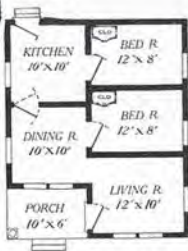
Floor Plan—The Thelma
