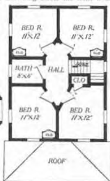
Second Floor Plan—The Virginia
