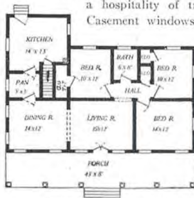
Floor Plan—The Kentucky
