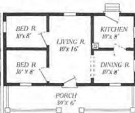
Floor Plan The Gretna No. 1.
