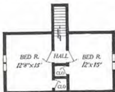
Second Floor Plan The Pomona with Second Story
