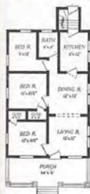
Floor Plan The Boulevard
