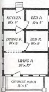
Floor Plan—The Leota
