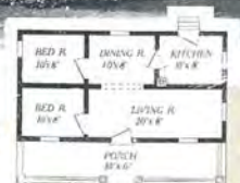
Floor Plan The Gretna No. 7
