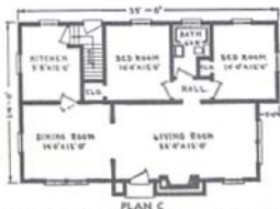
Plan "C" is size 35 x 24 feet over all. A wonderful 22-foot living room and large dining room feature this plan.
