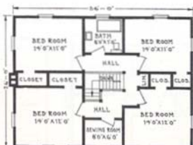
SECOND FLOOR PLAN—THE CAPITOL
