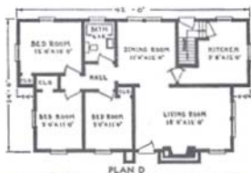
A beautiful three bedroom home, size 42 x 24 feet over all. Many buyers tell us they have saved a good thousand dollars or more on this home.
