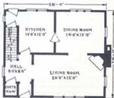
FIRST FLOOR PLAN No. 2
