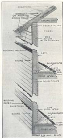
Construction of Aleddin Houses with Wall Sheathing and Sub-floor Shown
