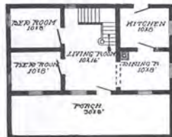
First Floor Plan, The Thorndale
