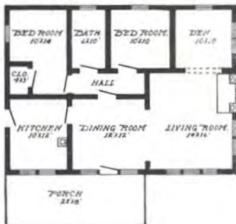
Floor Plan, The Royton
