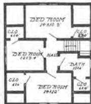
Second Floor Plan, The Marsden
