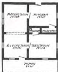
Floor Plan, The Hopeton. 26 x 32
