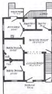
First Floor Plan, The Duplex
