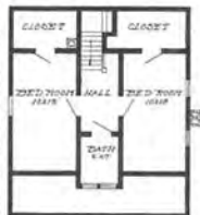
Second Floor Plan, The Detroit
