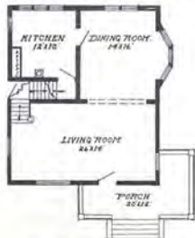
First Floor Plan, The Amherst
