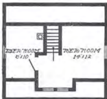
Second Floor Plan, The Jackson
