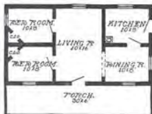
Floor Plan, The Gretna. 22 x 30
