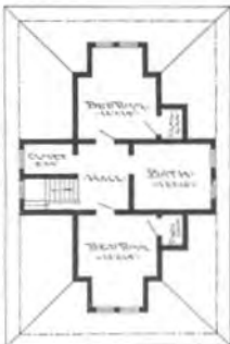
Second Floor Plan, The Albany
