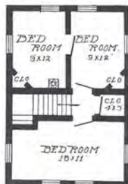
Second Floor Plan, The Finley
