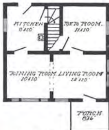
First Floor Plan, The Jackson
