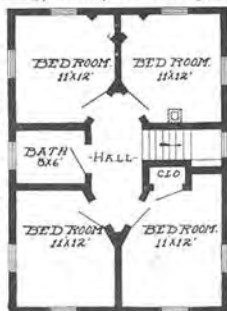
Second Floor Plan, The Virginia
