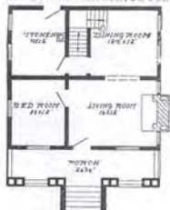
First Floor Plan, The Detroit
