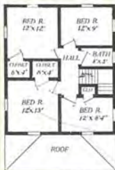
Second Floor Plan—The Hudson
