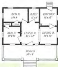
Floor Plan—The Edison
