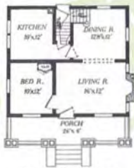
First Floor Plan—The Detroit
