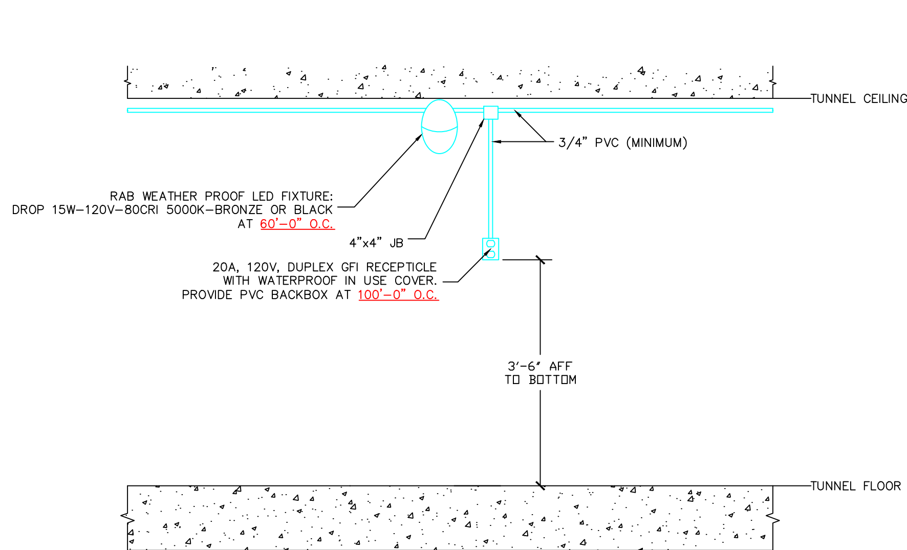
1 TUNNEL LIGHTING DETAIL G-1 SCALE: NTS
